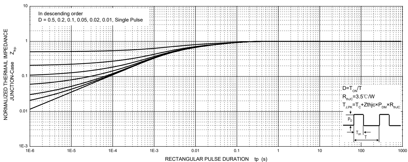
MUR20H20CT Transient Thermal Impedance, Junction-Case
