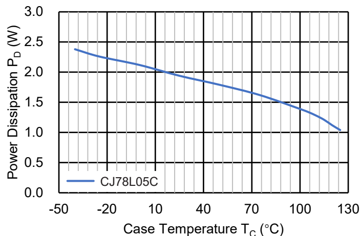
Power Dissipation
