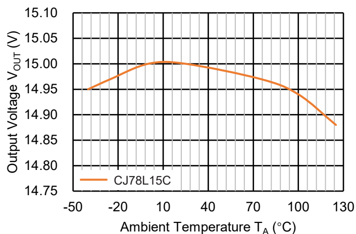
Temperature Characteristics
