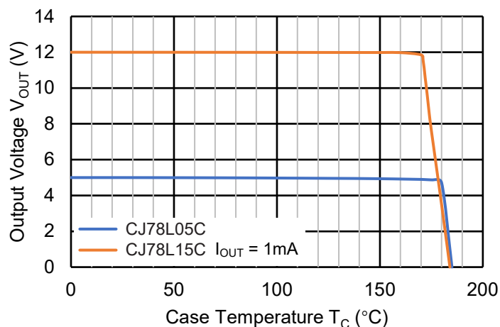
Thermal Shutdown
