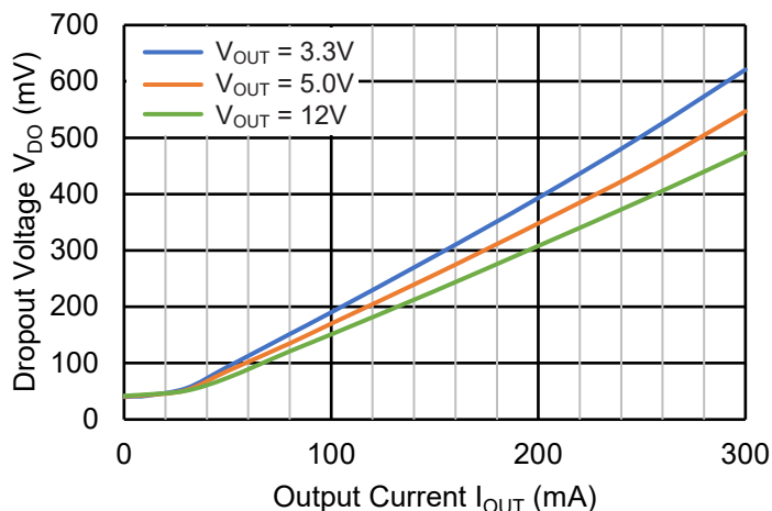
Dropout Voltage
