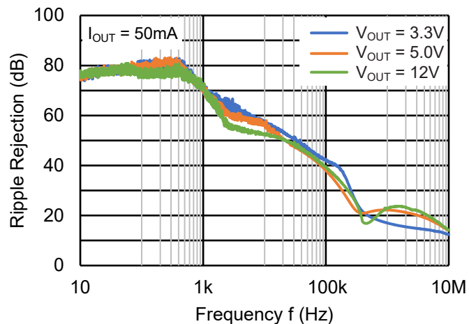
Ripple Rejection
