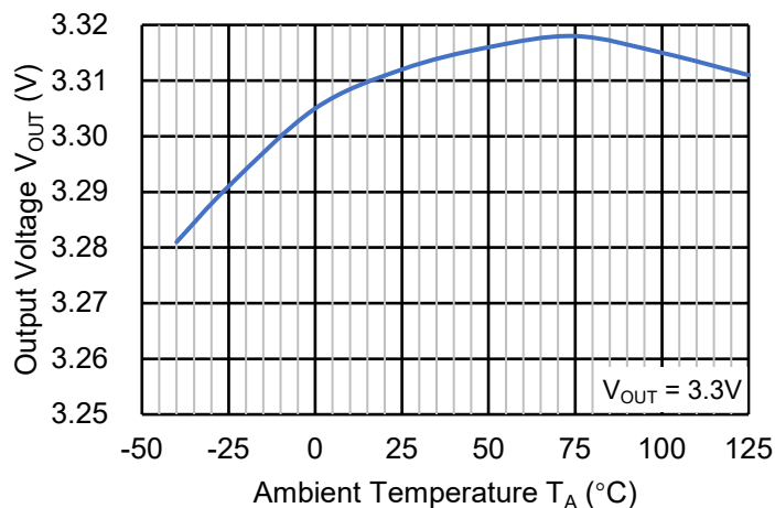
Temperature Characteristics
