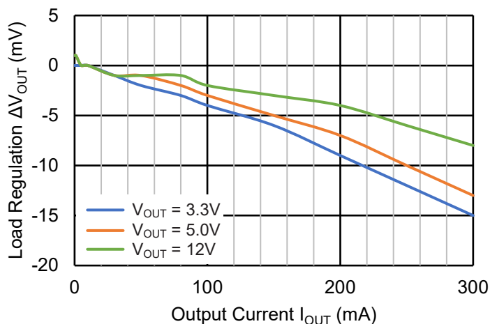
Load Regulation
