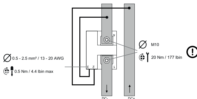
Fig. 8 Current (option B) and voltage inputs
