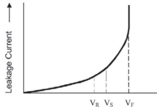
Figure 13 Leakage Current vs Voltage
