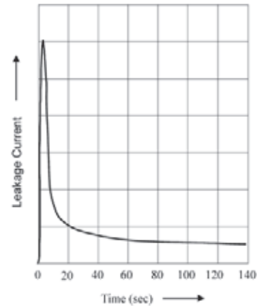
Figure 11 Time vs Leakage Current
