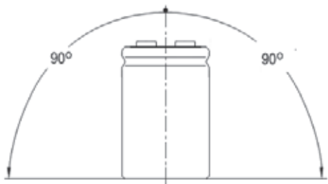
Figure 17 Recommended range of mounting positions
