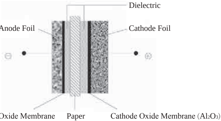
Figure 2 Cutting Construction of Aluminum Electrolytic Capacitor.
