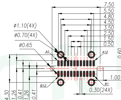
RECOMMENDED PCB LAYOUT(TOP VIEW) THICKNESS 1.0±0.10MM;DEFAULT TOLERANCE:±0.05
