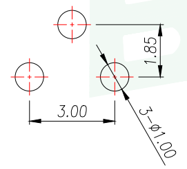
PCB.焊接图 PCB.WELDING DRAWING
