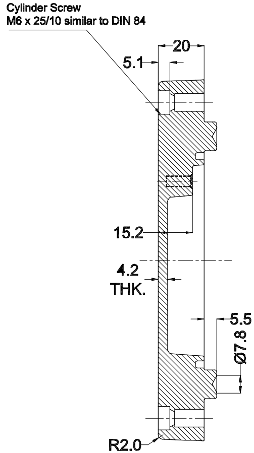
SECTION B-B
