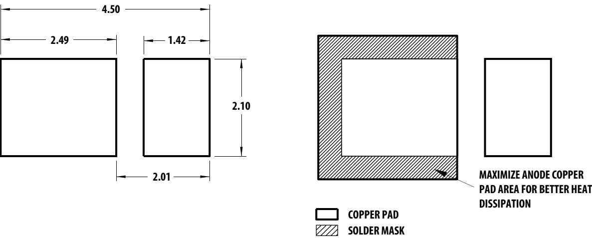
Figure 13 Recommended Soldering Land Pattern
