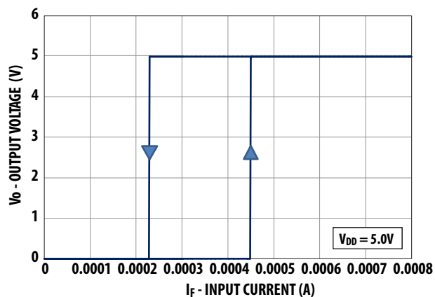
Figure 16: Output Voltage vs. Input Current at V_{DD} = 5\text{V}
