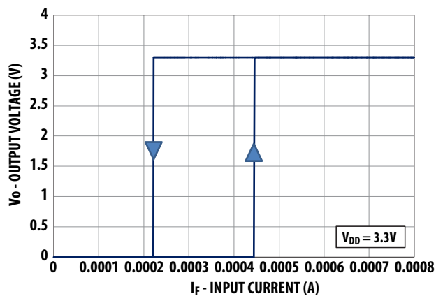
Figure 15: Output Voltage vs. Input Current at V_{DD} = 3.3\text{V}
