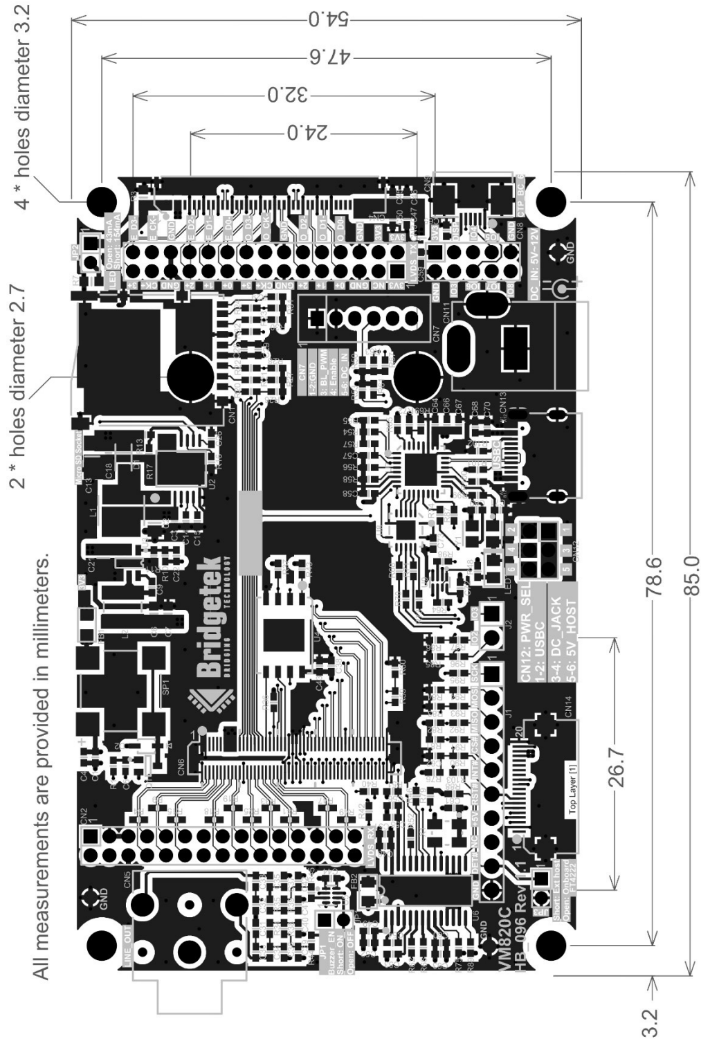
Figure 12 – VM820C PCB Dimensions
