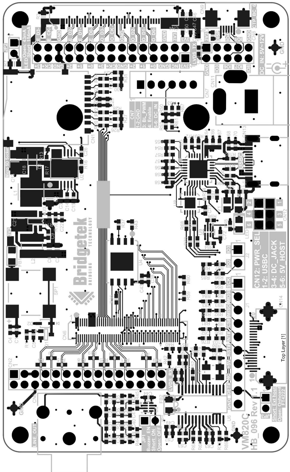
Figure 8 – Assembly Drawing
