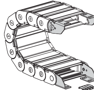
Fig. B Chain fixed outside/inside the radius. (Fig B)
