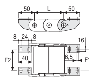
Fig. B Chain fixed outside/inside the radius. (Fig B)
