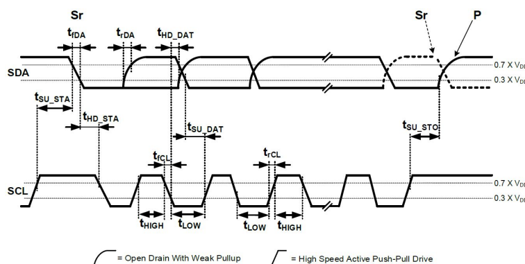
Figure 34: I 2 C timing diagram
