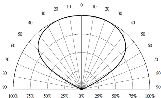
Radiation Diagram
