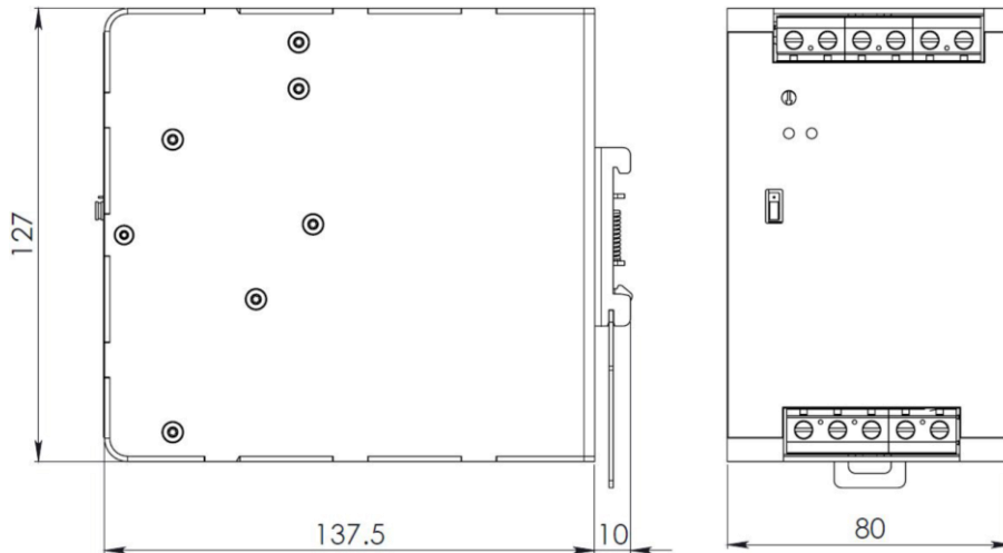
Figure 1. Mechanical Drawing
