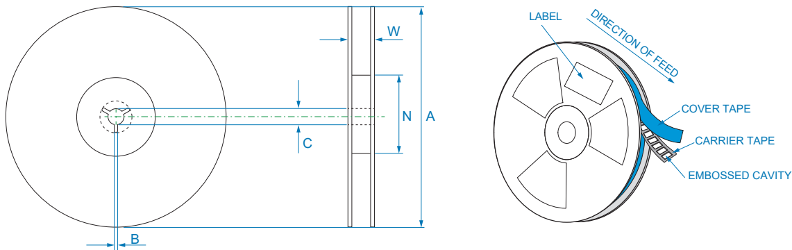
REEL DIMENSIONS (mm)
