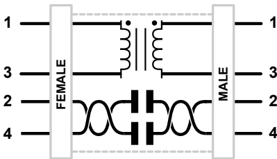
Wiring Diagram
