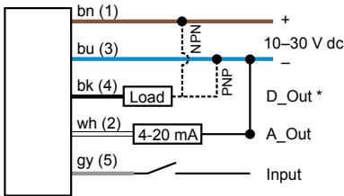
Push-pull Output and Analog Current Output
