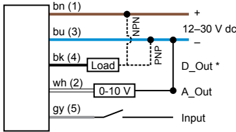
Push-pull Output and Analog Voltage Output
