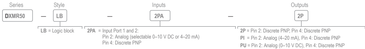
DXMR50-LB-2PA Ports
