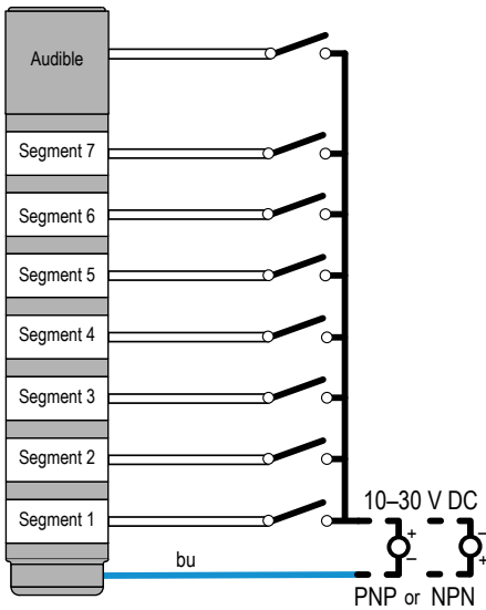
Wiring diagram for tower light application
