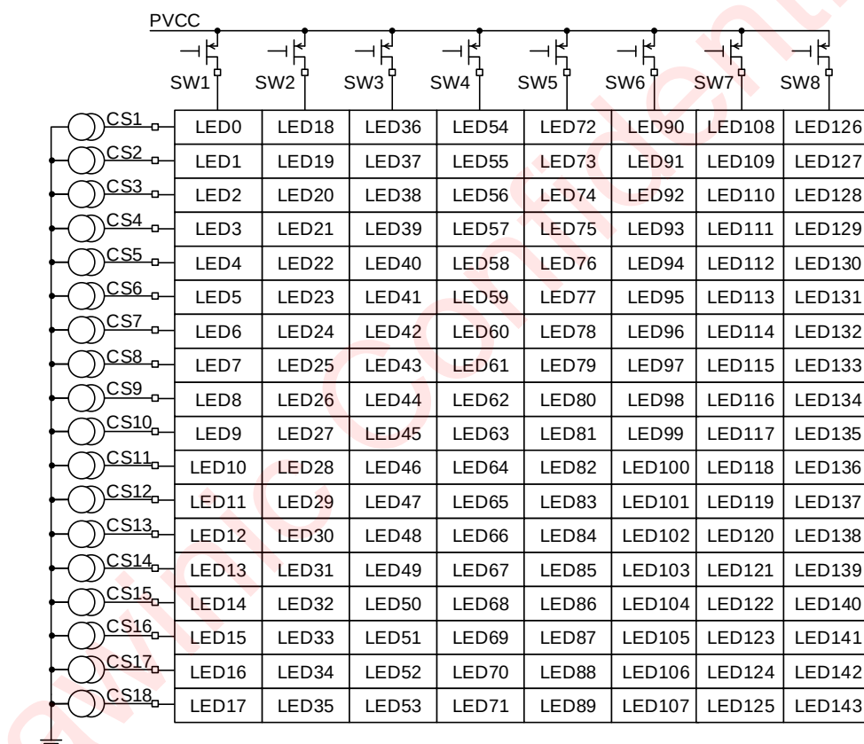
Figure 16 LED Location
