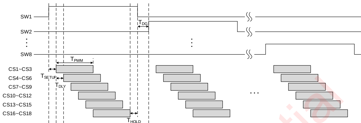
Figure 19 Scanning Timing
