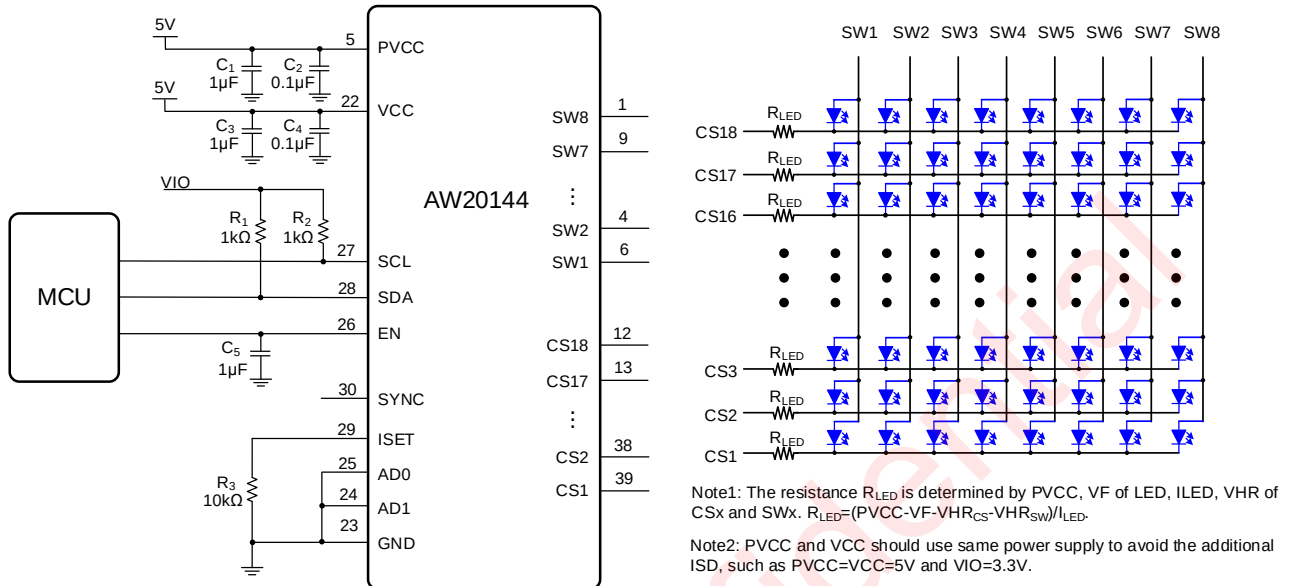
Figure 1 AW20144 Application Circuit
