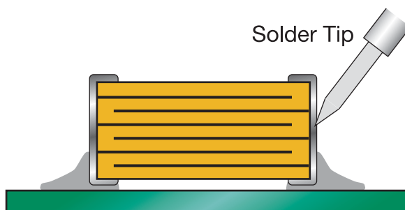
Poor Method - Direct Contact with Part
