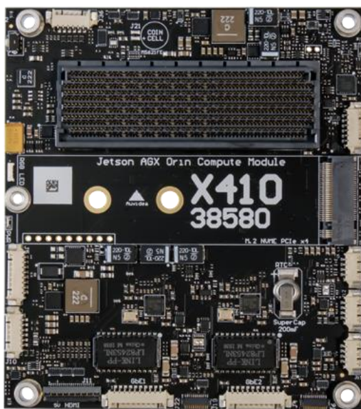
X410 top side
