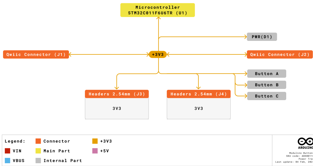
Modulino® Buttons Power Tree
