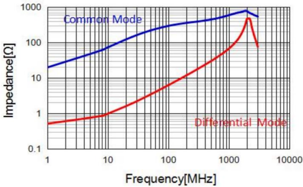
APCW3225-601P2T
