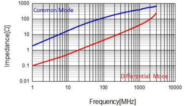
APCW2012-221P2T
