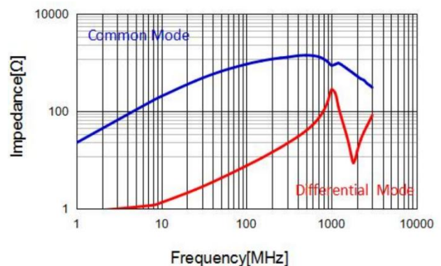
APCW4532-800P2T
