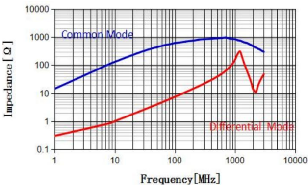
APCW3225-102P2T
