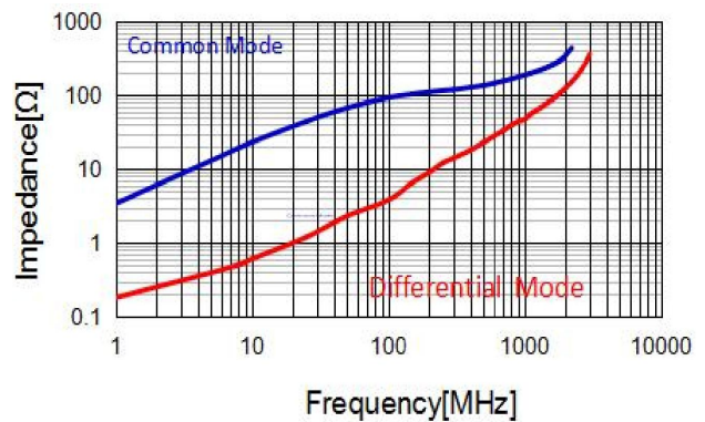
APCW4532-800P2T
