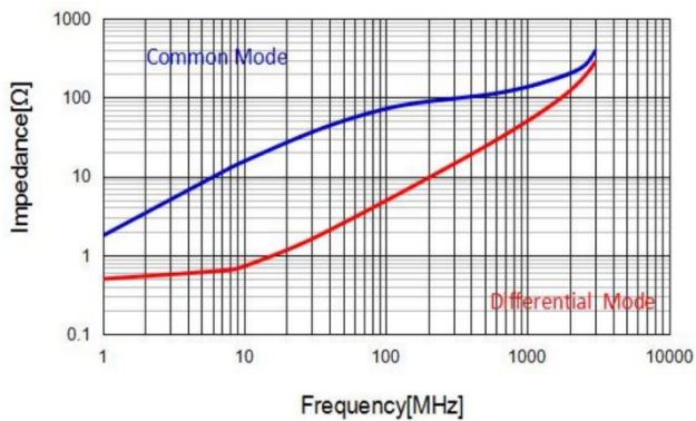
APCW3225-271P2T
