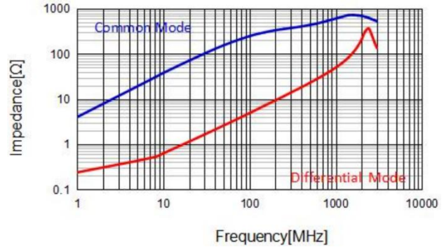
APCW2012-361P2T
