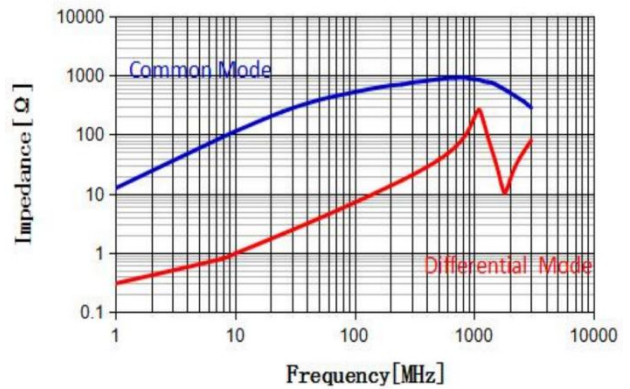
APCW3225-801P2T
