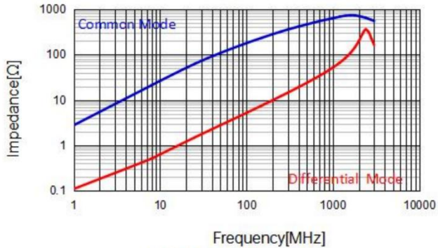
APCW2012-261P2T
