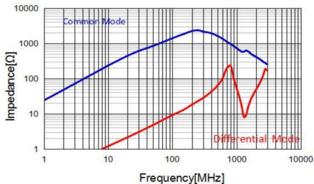
APCW4532-142P2T
