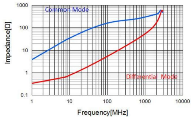
APCW3225-501P2T
