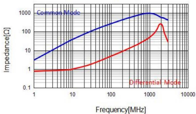
APCW2012-261P2T
