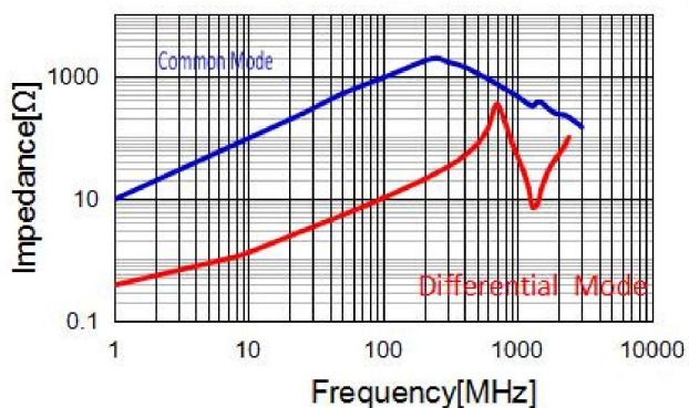
APCW4532-142P2T
