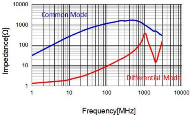
APCW3225-102P2T
