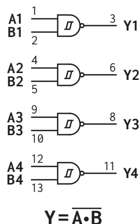
Figure 1: AF54RHC132 logic diagram
