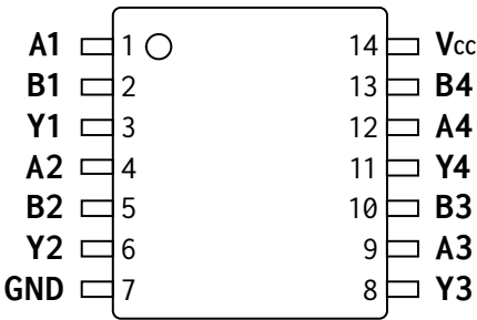
Figure 2: AF54RHC132 device pinout overview
