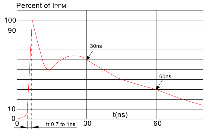
FIG.4: ESD clamping (8KV contact)
