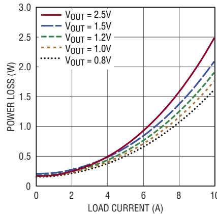
Figure 7. Power Loss vs Load Current at 3.3V IN
