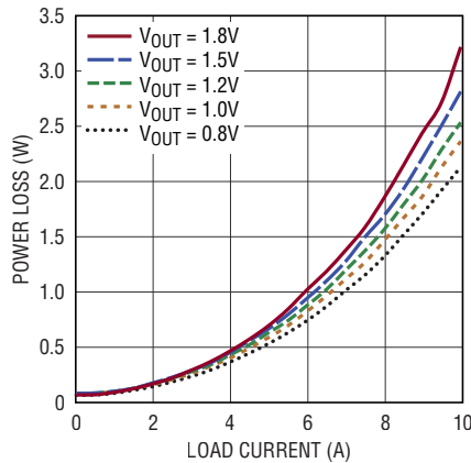
Figure 6. Power Loss vs Load Current at 2.5V IN
