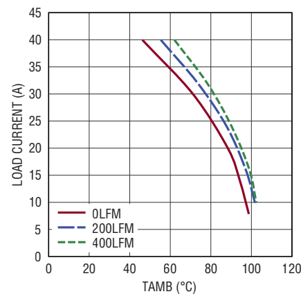
Figure 13. 5V to 1.5V Derating Curve, No Heat Sink
