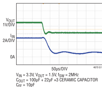
Short-Circuit with 10A Load
