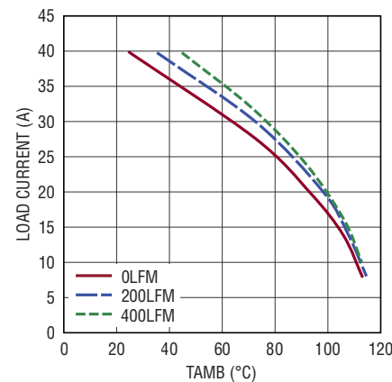
Figure 10. 3.3V to 1.5V Derating Curve, No Heat Sink
