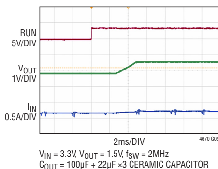
Start Into Prebiased Output
