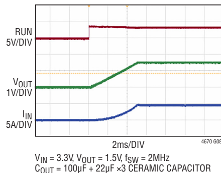
Start-Up with 10A Load
