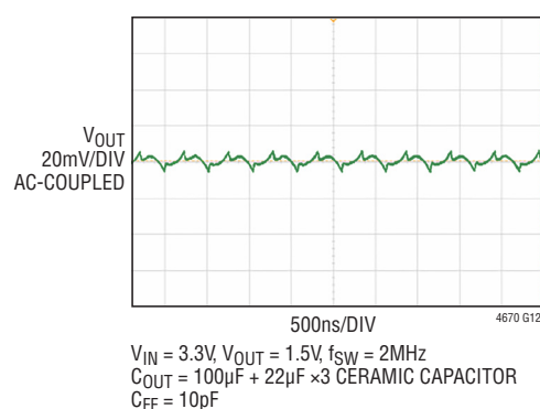
Steady State Voltage Ripple
