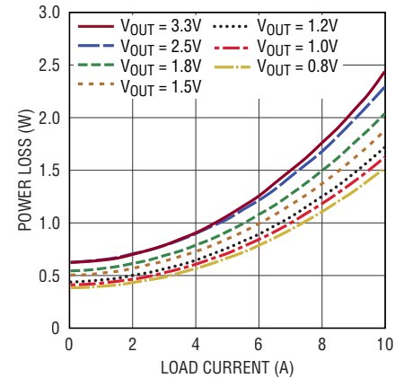
Figure 8. Power Loss vs Load Current at 5.5V IN
