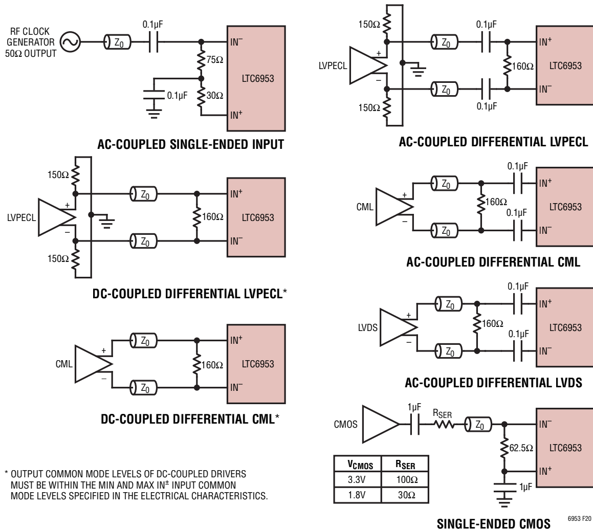
Figure 20. Common Input Interface Configurations. All Z_0 Signal Traces Are 50\Omega Transmission Lines
