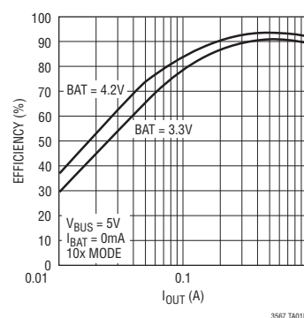
Switching Regulator Efficiency to System Load ( P_{OUT}/P_{BUS} )
