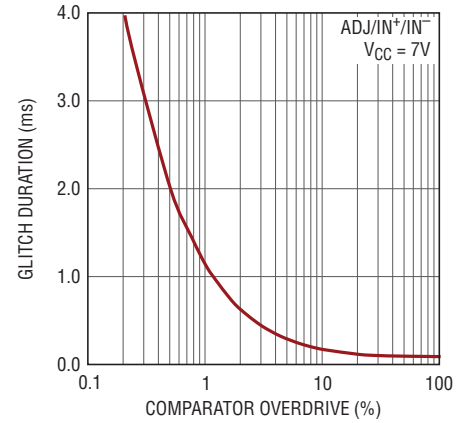
Comparator Overvoltage/Undervoltage Glitch Immunity
