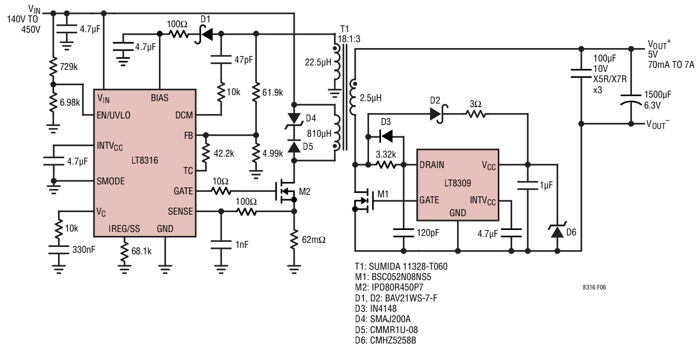
Figure 6. 91% Efficient Isolated 5V/7A Synchronous Flyback Converter
