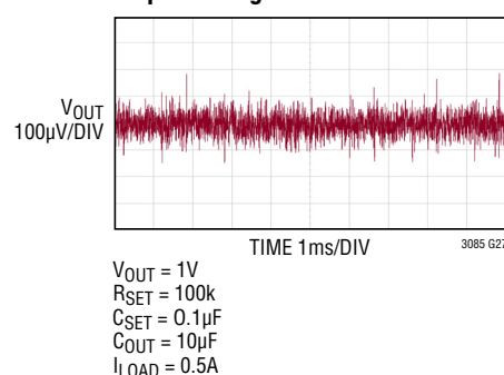
Output Voltage Noise
