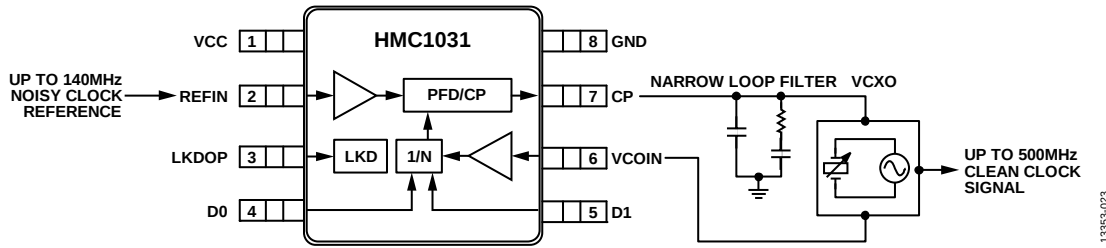
Figure 22. Typical Application Diagram
