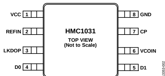
Figure 2. Pin Configuration
