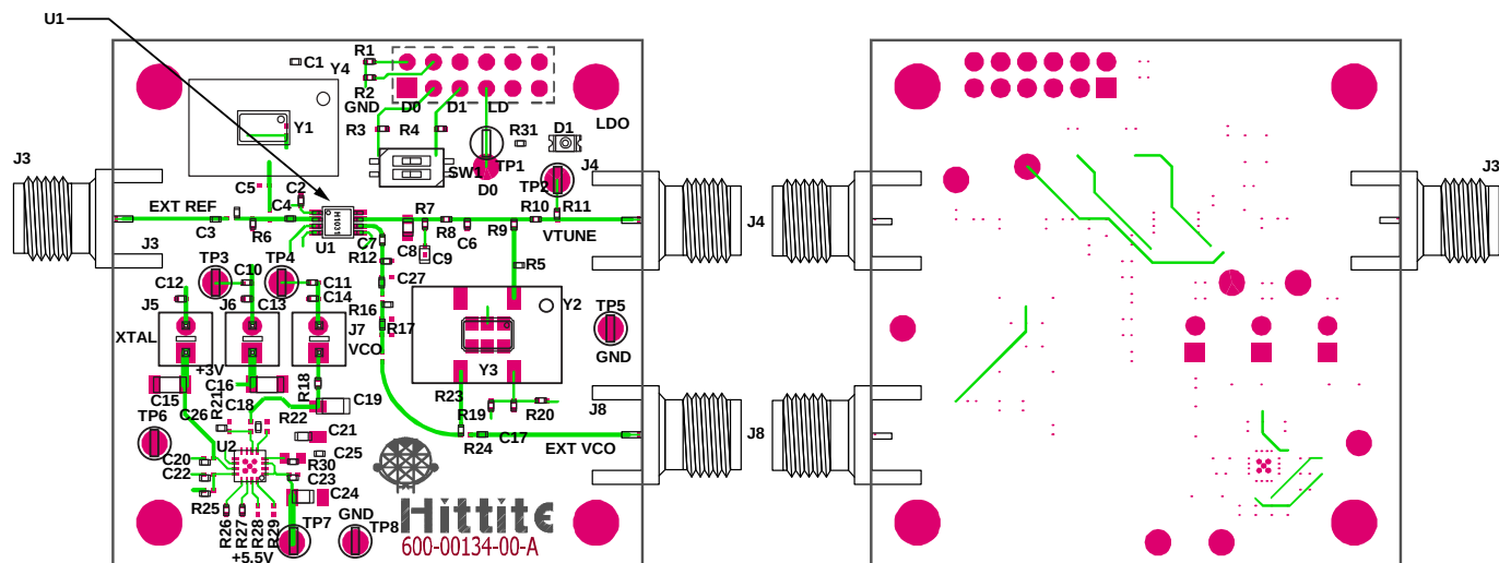
Figure 23. Evaluation PCB
