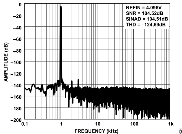
Figure 24. FFT, 2 MSPS, f_{IN} = 1\text{ kHz} , Differential Input = -0.5\text{ dBFS} , G = 1/3
