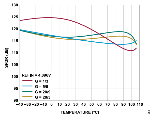
Figure 53. SFDR vs. Temperature, f_{IN} = 1 kHz, REF = 4.096 V
