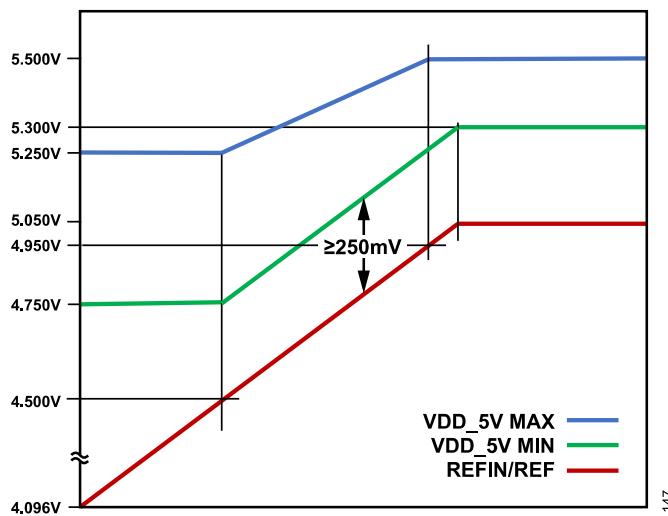
Figure 97. VDD_5V Minimum and Maximum Values for REFIN
