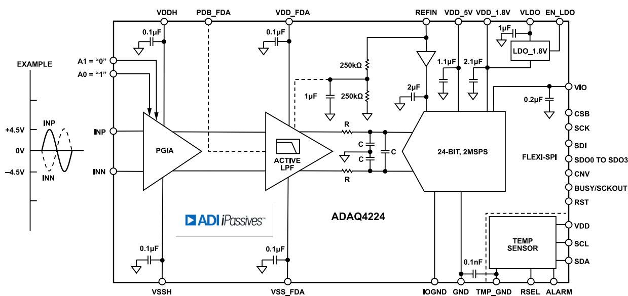
Figure 86. Differential Input Configuration with G = 5/9 V/V
