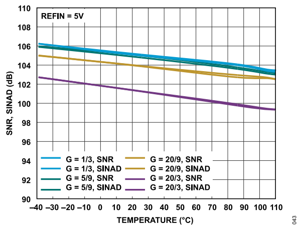
Figure 43. SNR, SINAD vs. Temperature, f_{IN} = 1 kHz Differential Input, REFIN = 5 V
