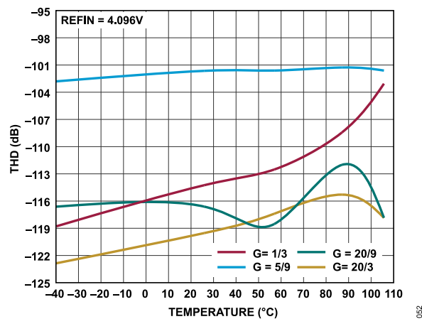
Figure 52. THD vs. Temperature, f_{IN} = 1 kHz Single-Ended Input, REF = 4.096 V
