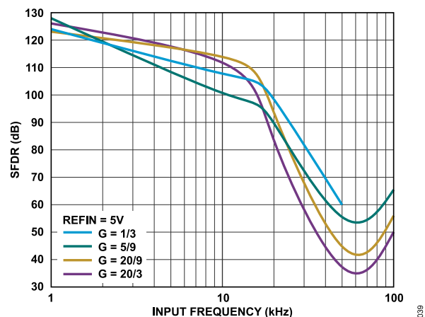
Figure 39. SFDR vs. Input Frequency, -0.5 \text{ dBFS} , \text{REFIN} = 5 \text{ V}
