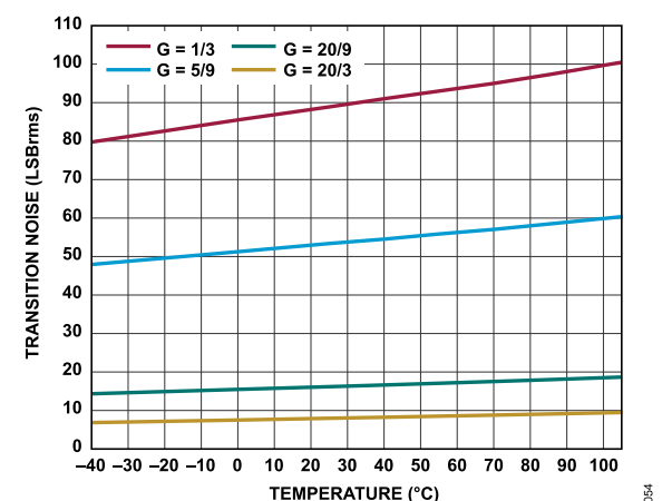
Figure 54. Transition Noise vs. Temperature, REF = 4.096 V
