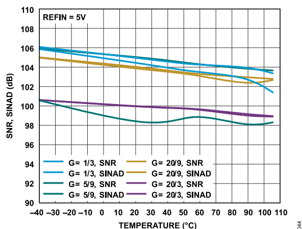
Figure 44. SNR, SINAD vs. Temperature, f_{IN} = 1 kHz Single-Ended Input, REFIN = 5 V
