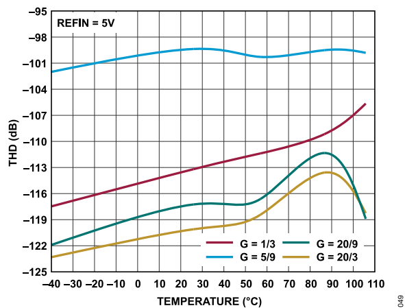
Figure 49. THD vs. Temperature, f_{IN} = 1 kHz Single-Ended Input, REF = 5 V
