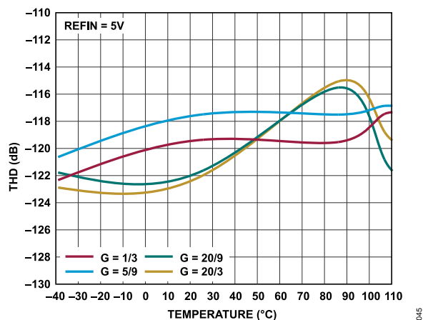
Figure 45. THD vs. Temperature, f_{IN} = 1 kHz Differential Input, REFIN = 5 V
