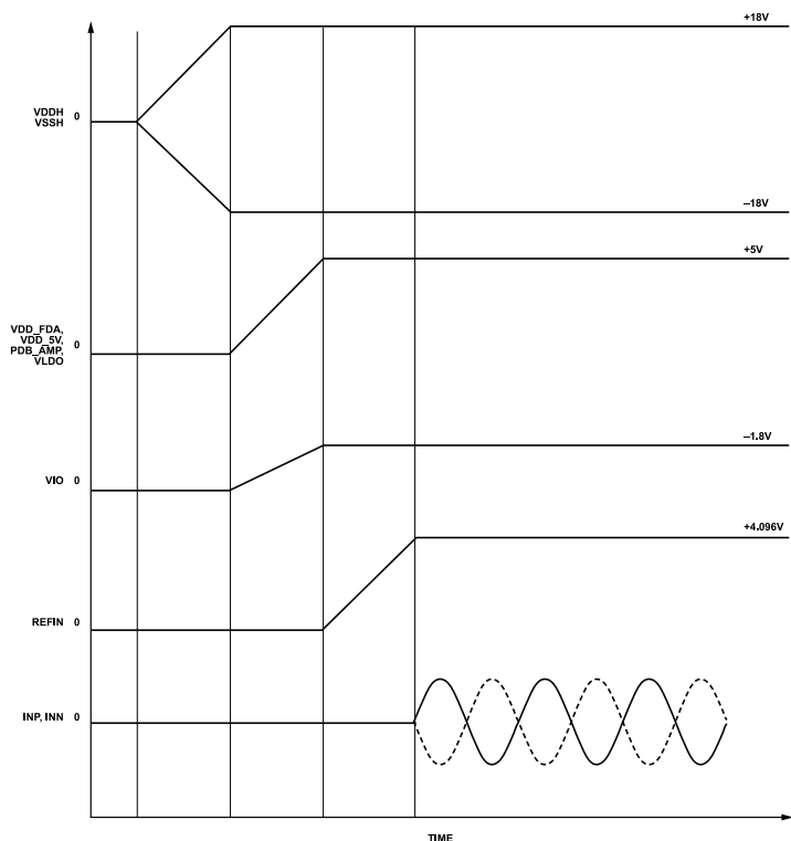
Figure 96. Power Supply Sequence
