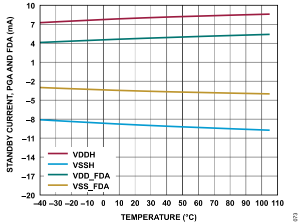
Figure 73. Standby Current PGA and FDA vs. Temperature
