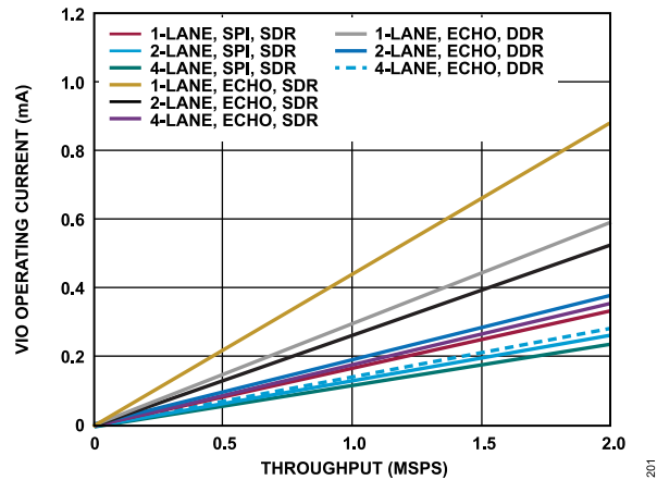
Figure 77. VIO Operating Current vs. Sample Rate
