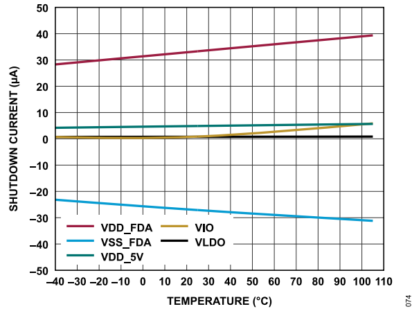
Figure 74. Shutdown Current vs. Temperature
