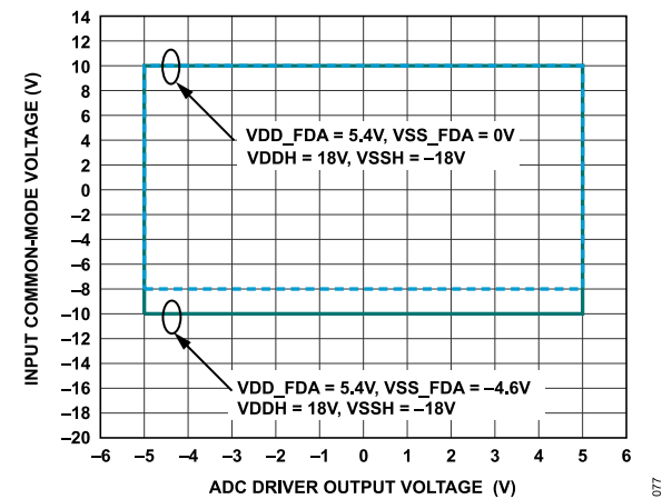
Figure 78. Input Common-Mode Voltage vs. ADC Driver Output Voltage, All Gains
