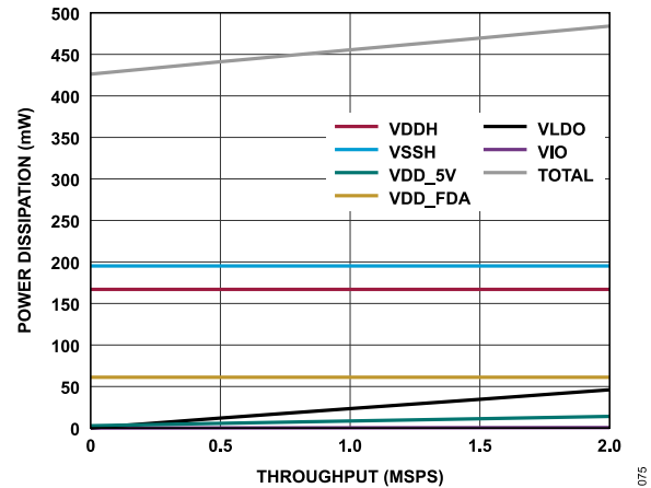
Figure 75. Power Dissipation vs. Throughput
