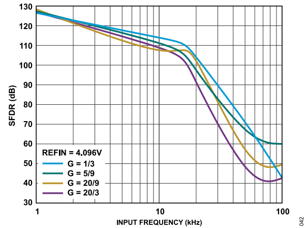
Figure 42. SFDR vs. Input Frequency, -0.5 \text{ dBFS} , \text{REFIN} = 4.096 \text{ V}
