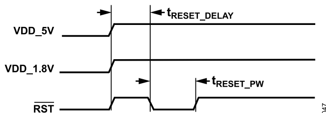
Figure 95. Power-On Reset (POR) Timing
