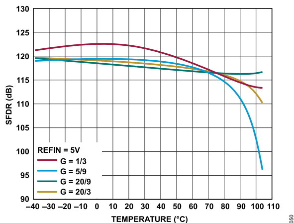
Figure 50. SFDR vs. Temperature, f_{IN} = 1 kHz, REF = 5 V
