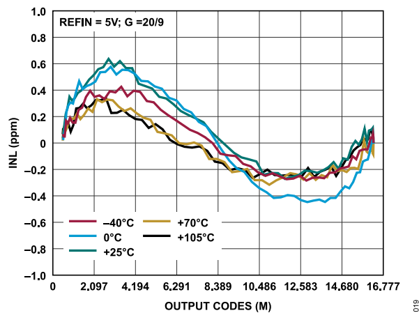
Figure 19. INL Error vs. Output Code across Temperature, G = 20/9
