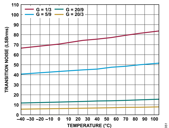
Figure 51. Transition Noise vs. Temperature, REF = 5 V
