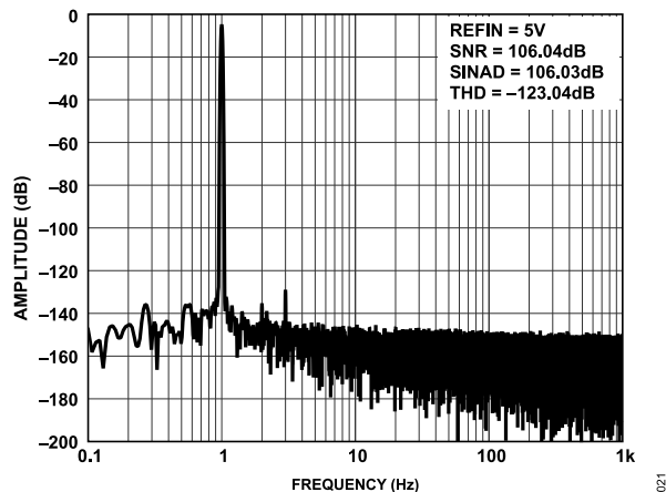
Figure 21. FFT, 2 MSPS, f_{IN} = 1\text{ kHz} , Differential Input = -0.5\text{ dBFS} , G = 1/3
