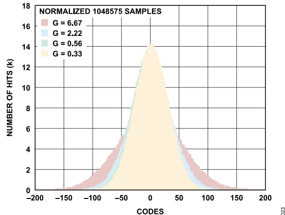
Figure 23. Code Histogram for Shorted Inputs, REFIN = 4.096\text{ V}
