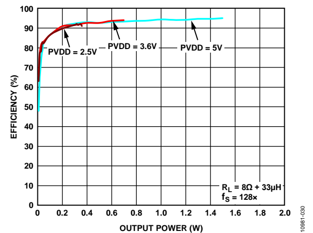
Figure 27. Efficiency vs. Output Power into 8\Omega , f_S = 128x
