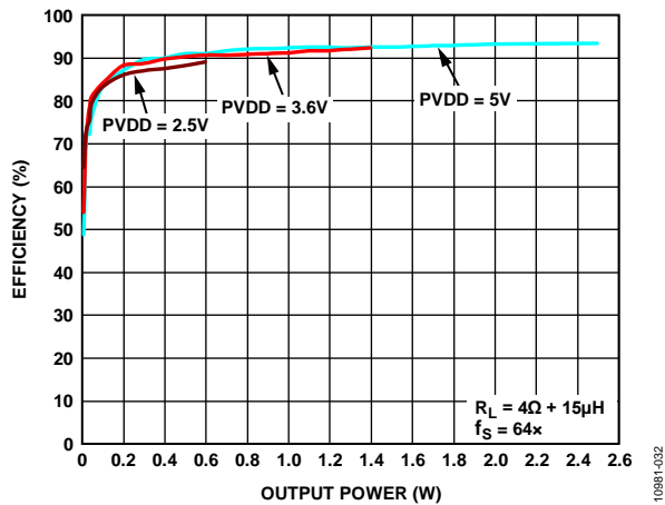
Figure 28. Efficiency vs. Output Power into 4\Omega , f_s = 64\times
