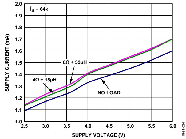
Figure 20. Quiescent Current vs. Supply Voltage, f_s = 64x
