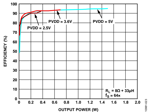
Figure 26. Efficiency vs. Output Power into 8\Omega , f_S = 64x
