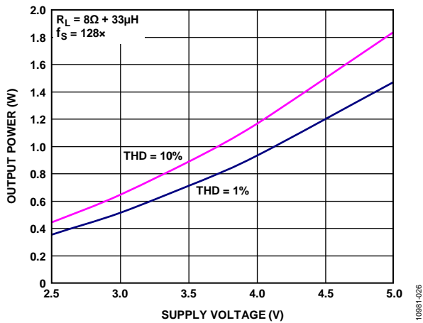
Figure 23. Maximum Output Power vs. Supply Voltage, R_L = 8\Omega , f_S = 128x
