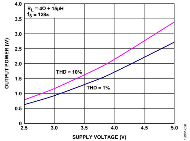
Figure 25. Maximum Output Power vs. Supply Voltage, R_L = 4\Omega , f_S = 128x
