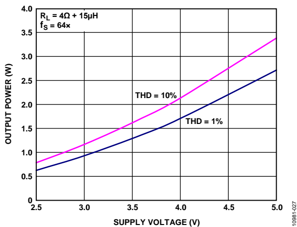
Figure 24. Maximum Output Power vs. Supply Voltage, R_L = 4\Omega , f_S = 64x
