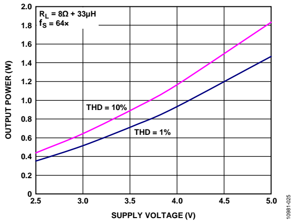
Figure 22. Maximum Output Power vs. Supply Voltage, R_L = 8\Omega , f_S = 64x
