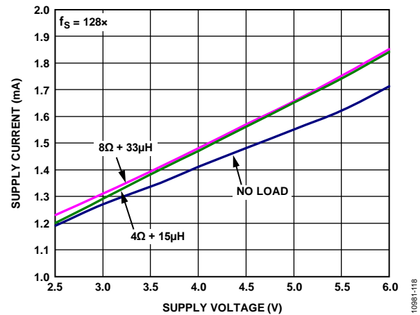
Figure 21. Quiescent Current vs. Supply Voltage, f_s = 128x
