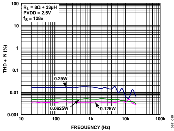
Figure 16. THD + N vs. Frequency, PVDD = 2.5V , R_L = 8\Omega , f_s = 128x
