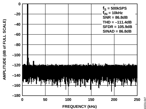
Figure 6. AD7988-5 FFT Plot, V_{REF} = 2.5\text{ V}
