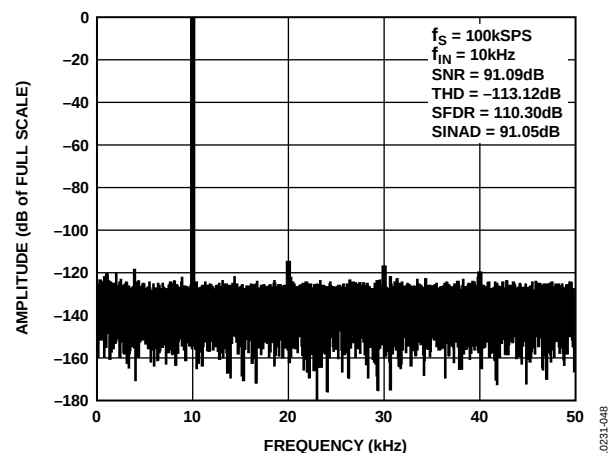
Figure 7. AD7988-1 FFT Plot, V_{REF} = 5\text{ V}
