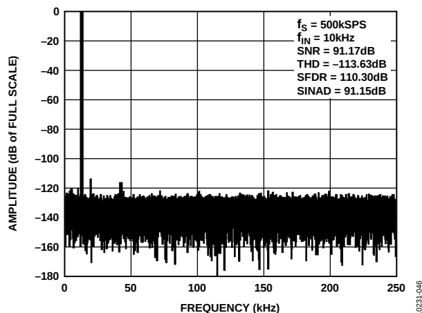
Figure 5. AD7988-5 FFT Plot, V_{REF} = 5\text{ V}
