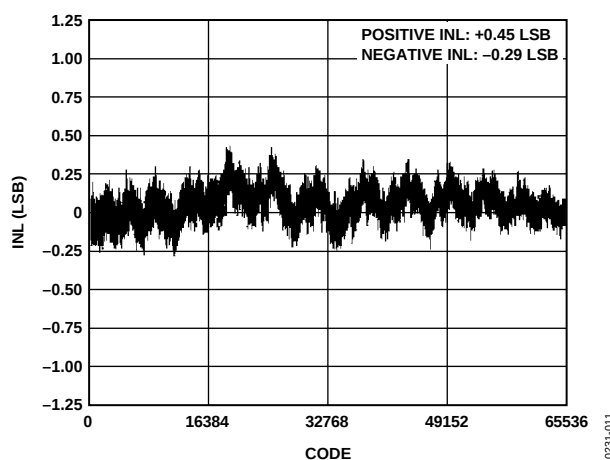
Figure 10. Integral Nonlinearity vs. Code, V_{REF} = 2.5\text{ V}
