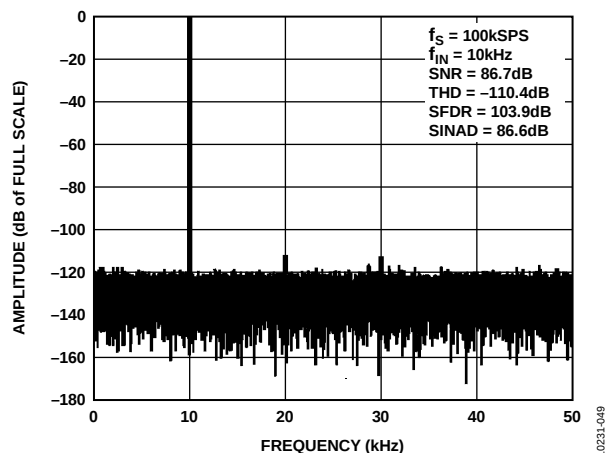
Figure 8. AD7988-1 FFT Plot, V_{REF} = 2.5\text{ V}
