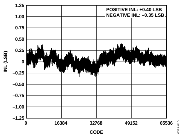
Figure 9. Integral Nonlinearity vs. Code, V_{REF} = 5\text{ V}
