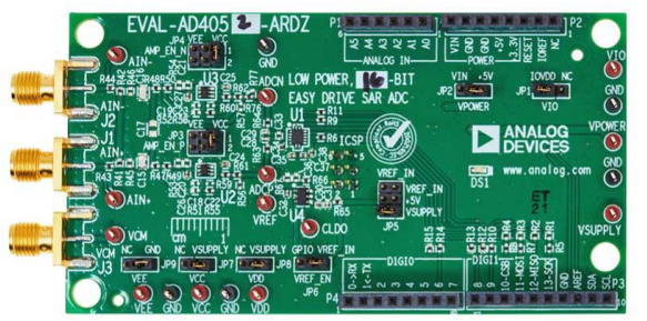
Figure 1. EVAL-AD4052-ARDZ Evaluation Board Photograph
