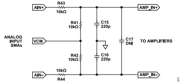
Figure 11. Signal and Common-Mode Inputs and Input Filter
