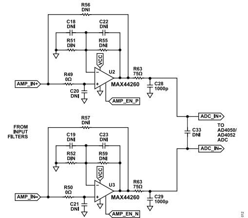
Figure 12. Default Amplifier Circuit Simplified Schematics
