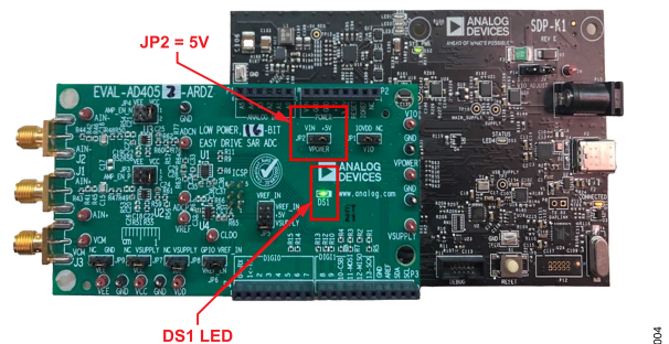
Figure 4. EVAL-AD4052-ARDZ on USB Power
