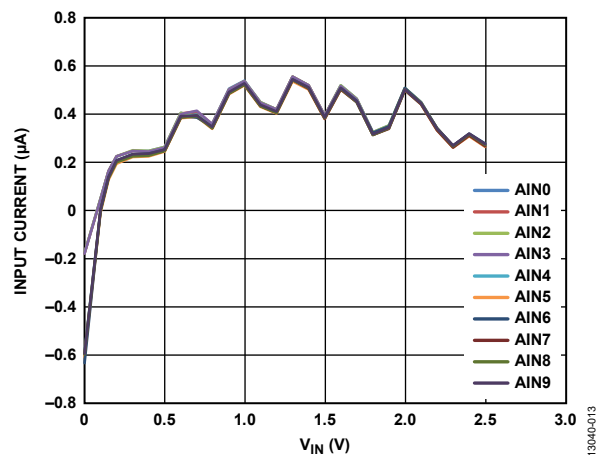
Figure 13. Input Current vs. V_{IN} , V_{DD} = 3.3\text{ V} , T_A = 25^\circ\text{C} , Unbuffered Mode, 100 KSPS
