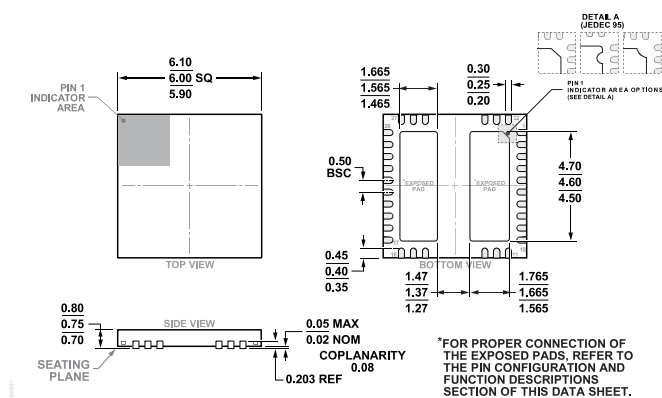
Figure 37. 32-Lead Lead Frame Chip Scale Package [LFCSP] 6 mm × 6 mm Body and 0.75 mm Package Height (CP-32-32) Dimensions shown in millimeters
