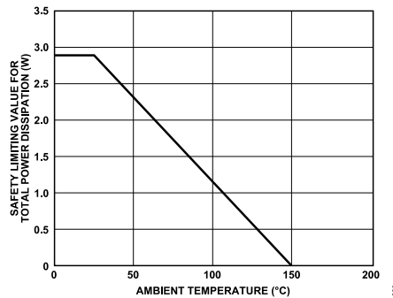
Figure 2. Thermal Derating Curve, Dependence of Safety Limiting Values with Ambient Temperature per DIN V VDE V 0884-11, SOIC_W_FP
