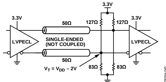
Figure 39. LVPECL DC-Coupled Termination
