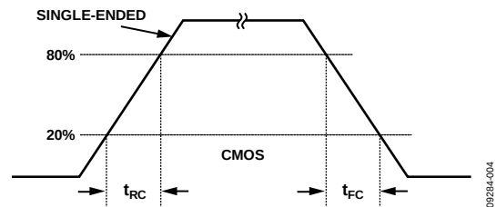
Figure 4. CMOS Timing, Single-Ended, 5 pF Load
