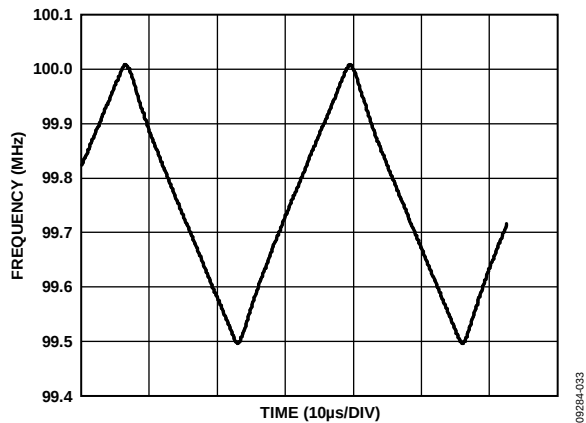
Figure 29. Typical Spread Spectrum Frequency Modulation Profile OUT2, N_b = 96 , FRAC = 0 , MOD = 1000 , CkDiv = 7 , NumSteps = 59 , FracStep = -8 , f_{OUT} = 100 MHz with -0.5\% Downspread at 30.2 kHz, MAX\_BW set to 0
