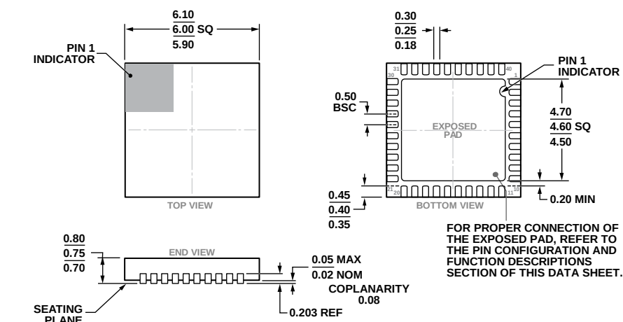
Figure 51. 40-Lead Lead Frame Chip Scale Package [LFCSP_WQ] 6 mm × 6 mm Body, Very Very Thin Quad (CP-40-7)
