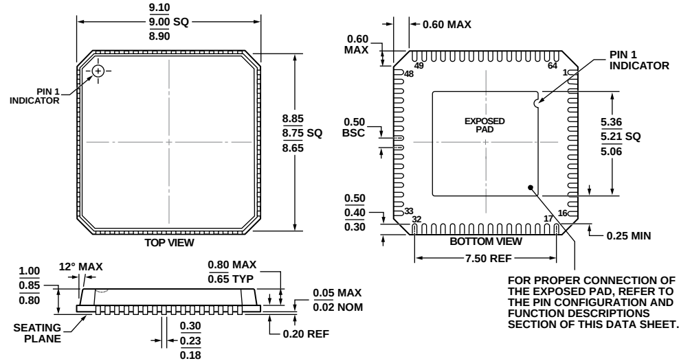
COMPLIANT TO JEDEC STANDARDS MO-220-VMMD-4 Figure 60. 64-Lead Lead Frame Chip Scale Package [LFCSP_VQ] 9 mm x 9 mm Body, Very Thin Quad (CP-64-7) Dimensions shown in millimeters
