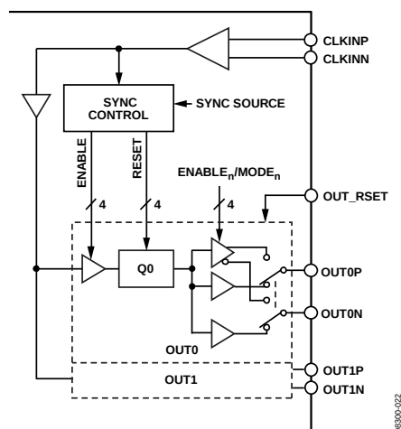
Figure 47. Clock Distribution
