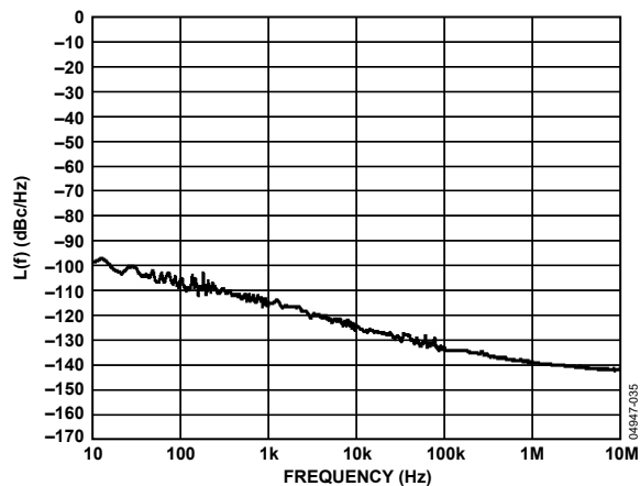
Figure 28. RF Divider and CML Driver Residual Phase Noise (2488 MHz In, 622 MHz Out)
