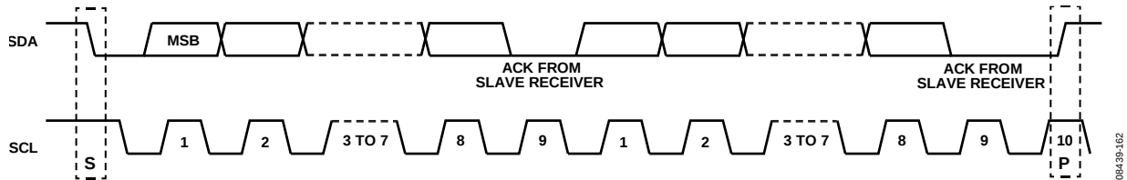
Figure 32. Data Transfer Process (Master Write Mode, 2-Byte Transfer)
