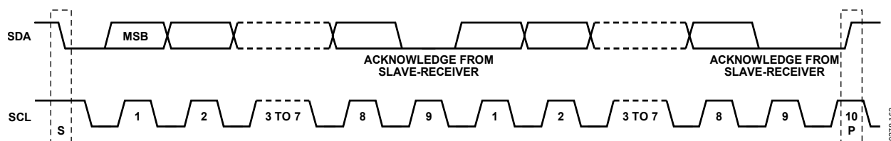
Figure 34. Acknowledge Bit
