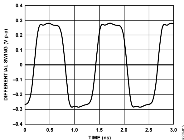
Figure 17. LVDS Differential Voltage Swing at 800 MHz Output Terminated 100 \Omega Across Differential Pair
