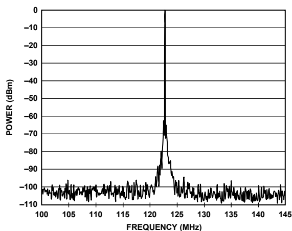
Figure 13. PFD/CP Spurs; 122.88 MHz; PFD = 15.36 MHz; LBW = 127 kHz; I_{CP} = 3.0 mA; f_{VCO} = 1475 MHz
