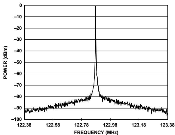
Figure 14. Output Spectrum, LVDS; 122.88 MHz; PFD = 15.36 MHz; LBW = 127 kHz; I_{CP} = 3.0 mA; f_{VCO} = 1475 MHz
