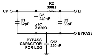
Figure 42. Typical PLL Loop Filter Used for Clock Generation
