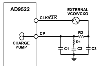
Figure 41. Example of External Loop Filter for a PLL Using an External VCO
