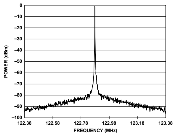
Figure 14. Output Spectrum, LVDS; 122.88 MHz; PFD = 15.36 MHz; LBW = 127 kHz; I_{CP} = 3.0 mA; f_{VCO} = 2458 MHz
